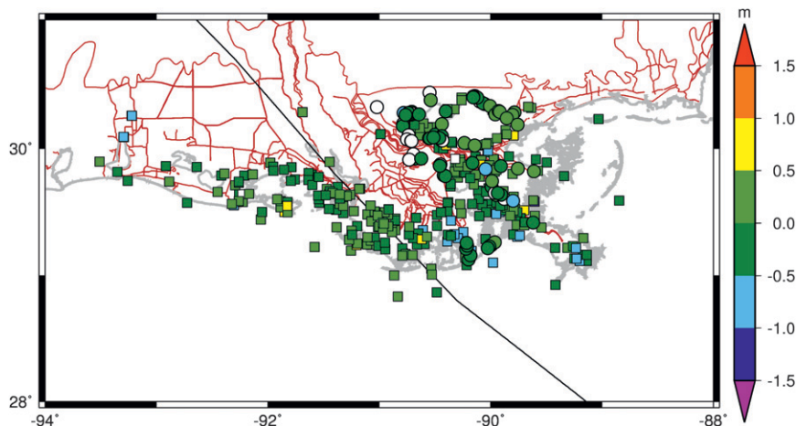
FIG. 28. Locations of the 82 URS/FEMA HWMs (circles) and 362 hydrographs (squares) in southeastern Louisiana. The points are color-coded to show the errors (modeled less measured) between the peak water levels; green points indicate matches within 0.5 m. Warm colors indicate locations where ADCIRC overpredicted the peak water level, while cool colors indicate locations where ADCIRC underpredicted the peak water level. White points indicate locations that were never wetted by ADCIRC.
