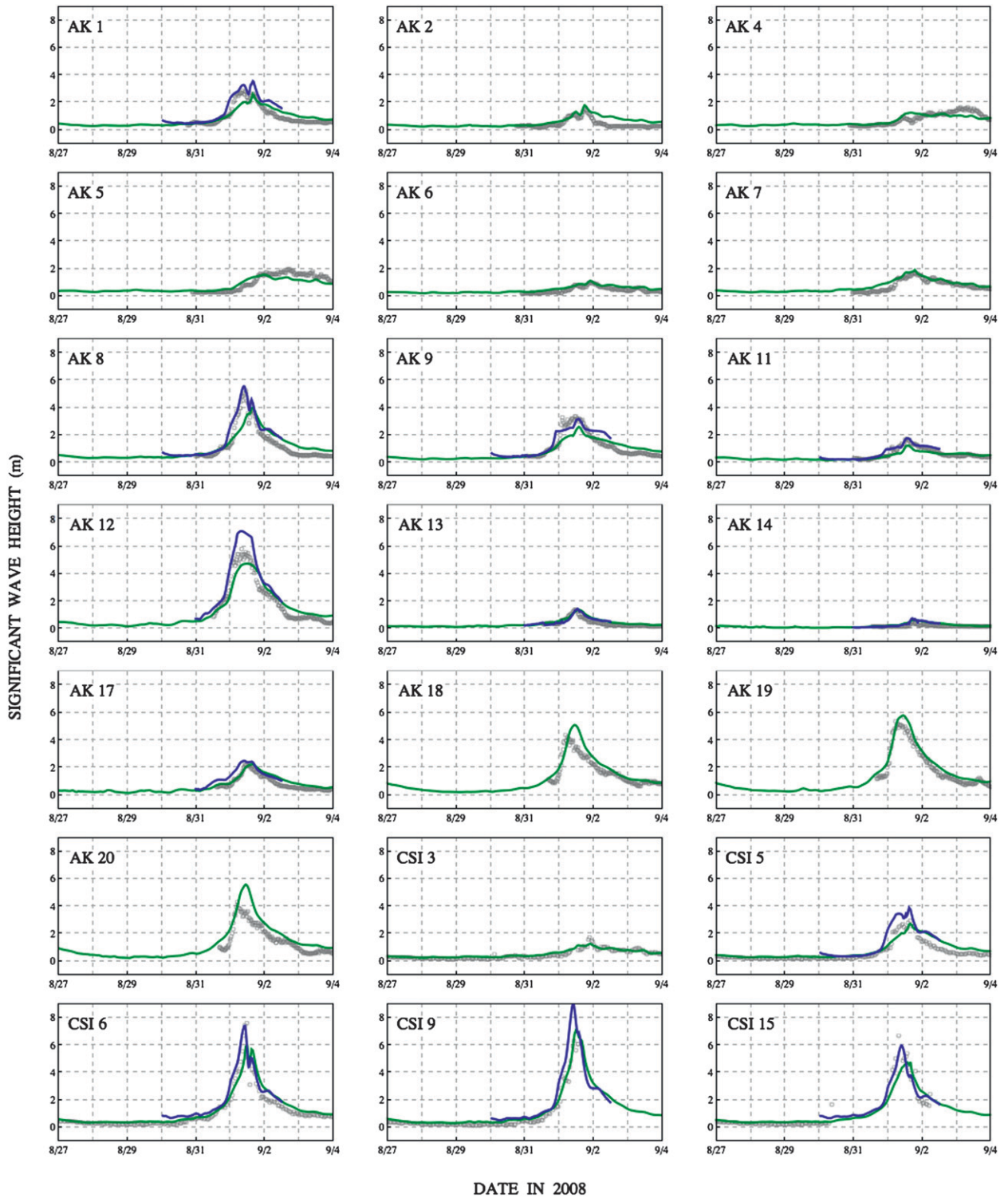
FIG. 17. Time series of significant wave heights (m) at the 16 AK gauges and five CSI gauges shown in Fig. 16. Measured values are shown with gray circles; modeled results from SWAN (green) and STWAVE (blue) are shown with solid lines.
